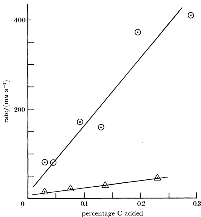
FIGURE 2. Results of 'feeding' experiments where fresh plankton ( \odot ) and plankton degraded oxically for 72 days ( \triangle ) were each added to Long Island Sound sediment samples in varying amounts. Rate refers to rate of sulphate reduction as determined by using a ^{35}\text{S} tracer. Data from Westrich & Berner (1984). (See also Berner 1984.)
