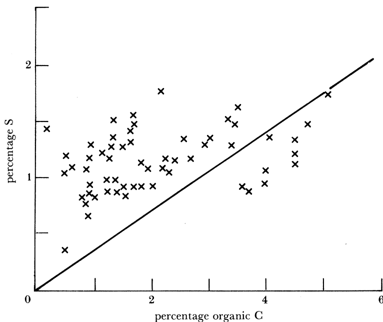
FIGURE 5. Plot of pyrite sulphur against organic carbon for euxinic, deep-water sediments of the Black Sea. Data from Rozanov et al. (1974). The straight line is the regression line for normal marine sediments taken from figure 4. After Berner (1984).
